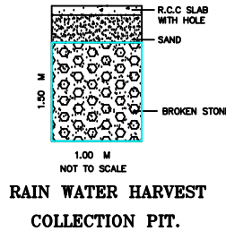
RAIN WATER HARVEST COLLECTION PIT.
