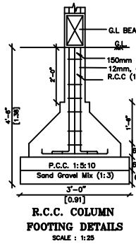
R.C.C. COLUMN FOOTING DETAILS
