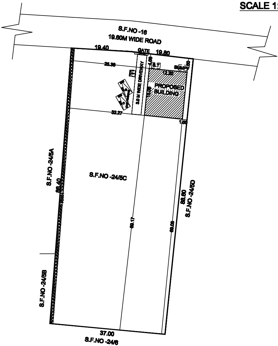
SITE PLAN
