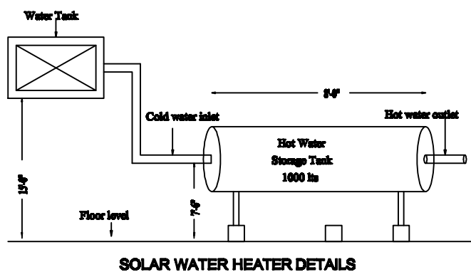
SOLAR WATER HEATER DETAILS
