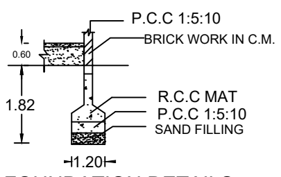
FOUNDATION DETAILS
