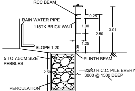
RAINWATER HARVESTING
