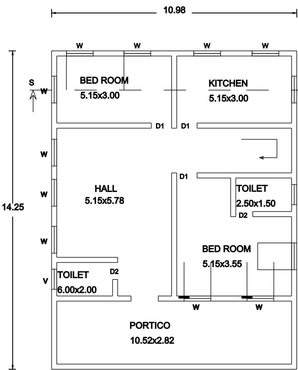
GROUND FLOOR
