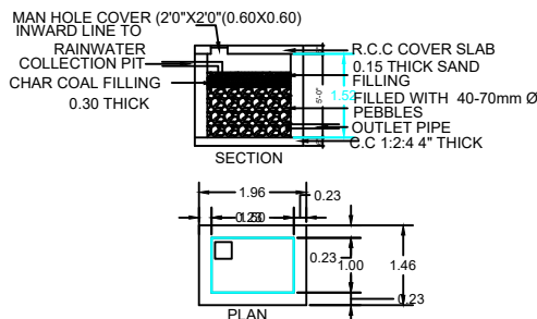
RWH_CAPACITY_L=5000LTRS DETAILS OF COLLECTION SUMP FOR RAIN WATER HARVESTING OF ROOF TOP RAIN WATER
