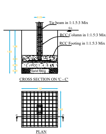
COLOUMN FOUNDATION DETAILS
