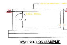
RWH_CAPACITY_L = 2000LTRS
