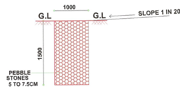
SECTION OF PEBBLE TRENCH SCALE : 1: = 100
