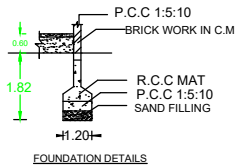
FOUNDATION DETAILS
