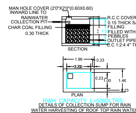
RAINWATER HARVESTING
