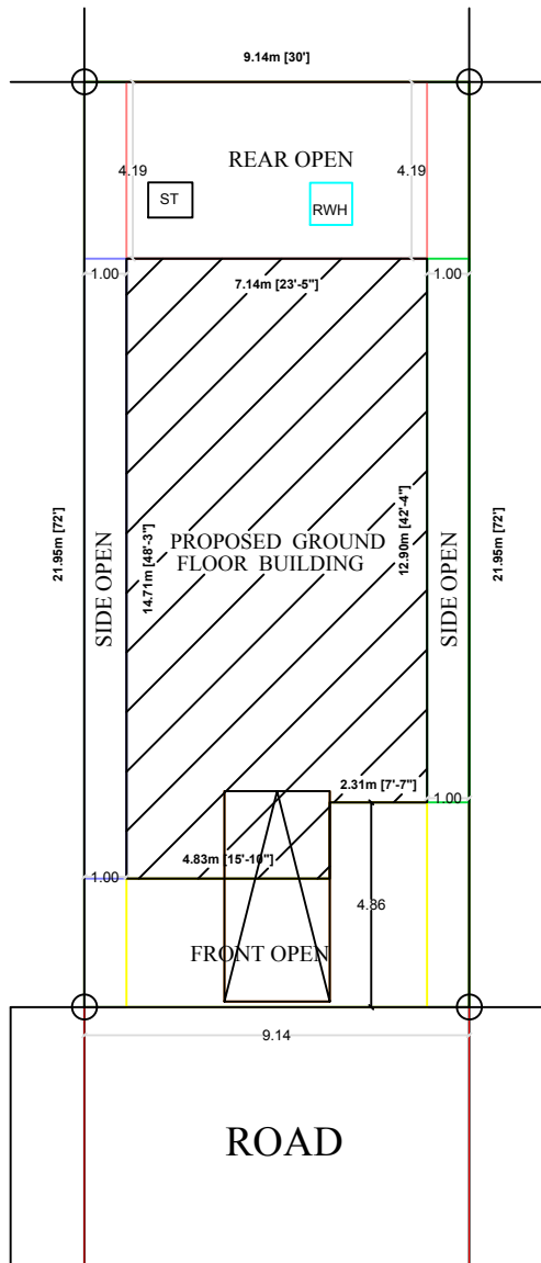
SITE PLAN
