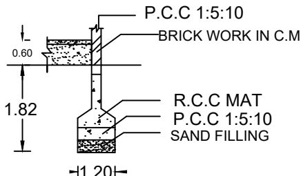
FOUNDATION DETAILS
