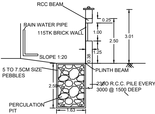
RAINWATER HARVESTING
