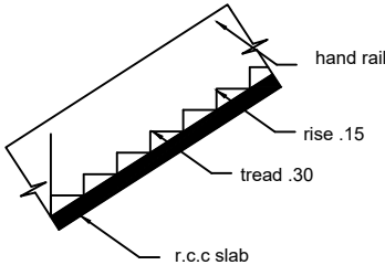
STAIR
