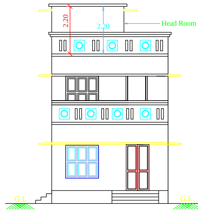
FRONT ELEVATION
