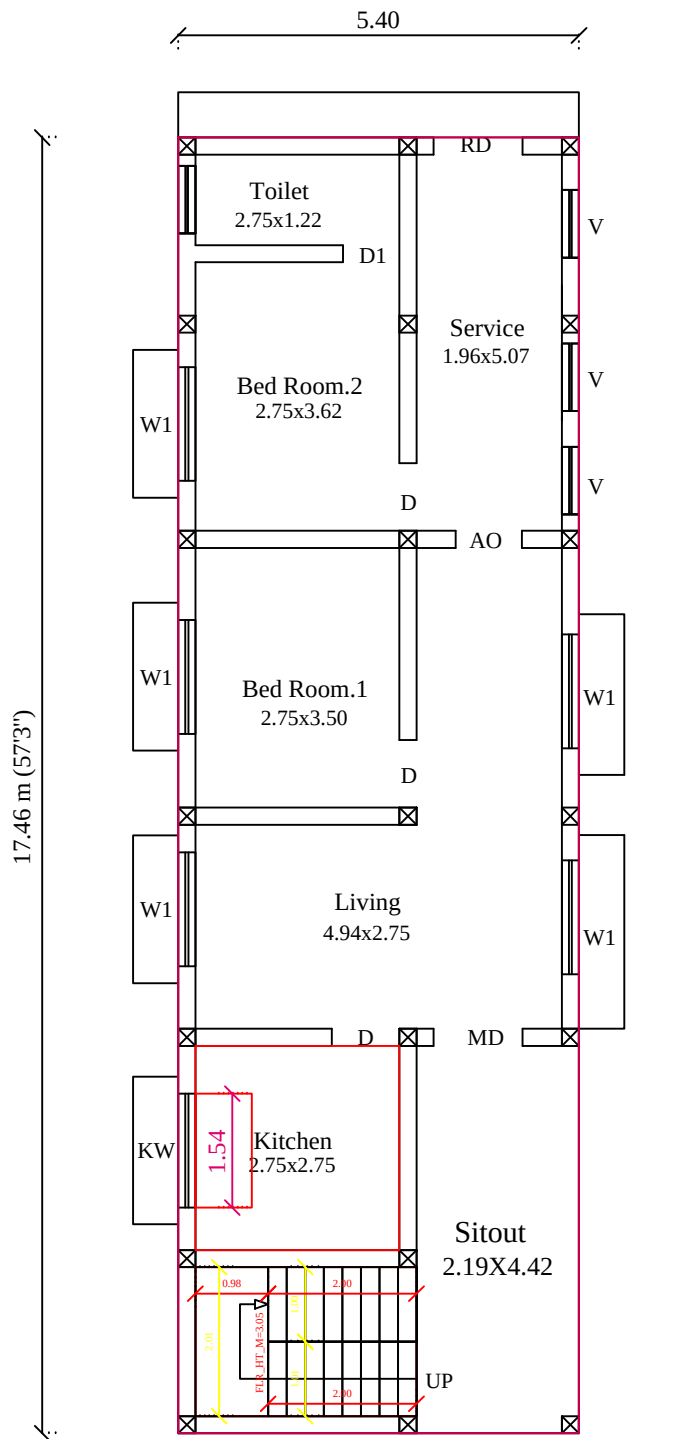
EXISTING GROUND FLOOR PLAN FACING EAST
