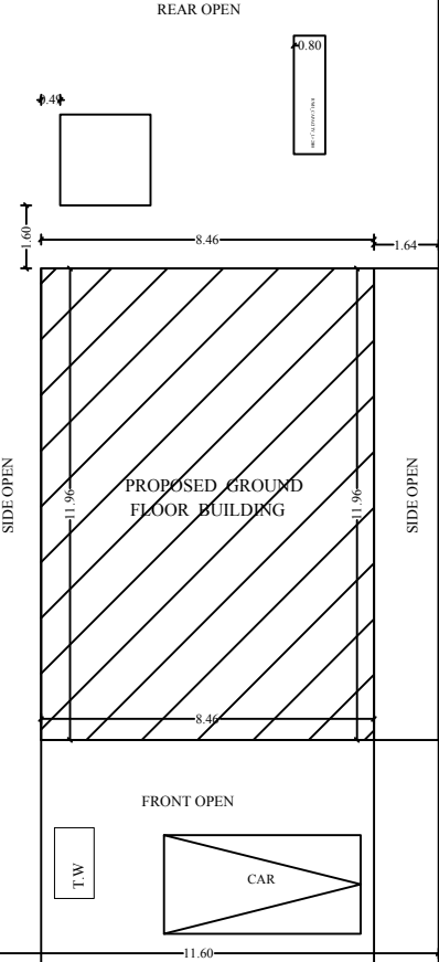
SITE PLAN
