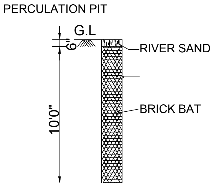
PERCOLATION PIT
