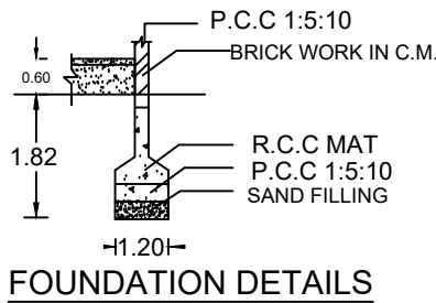
FOUNDATION DETAILS
