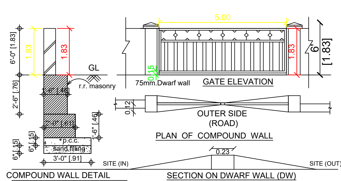
COMPOUND WALL DETAIL
