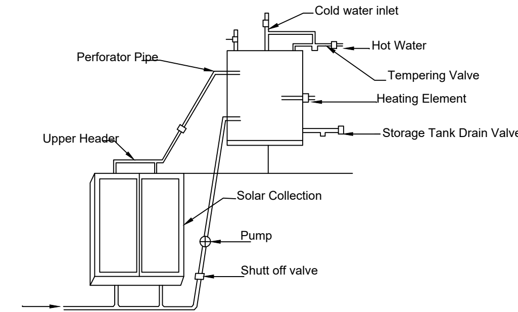
Details of solar water Heater (NTS)
