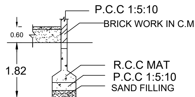
FOUNDATION DETAILS
