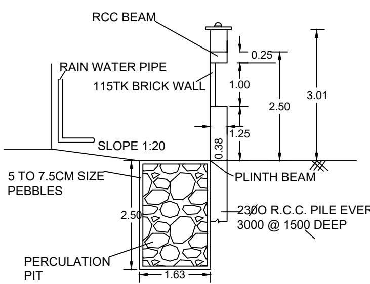
RAINWATER HARVESTING
