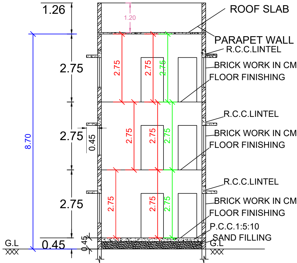
SECTION ON SS
