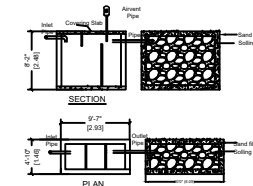
DETAILS OF SEPTIC TANK & DISPERSION TRENCH
