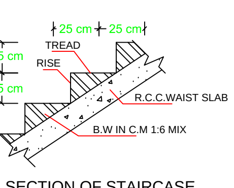
SECTION OF STAIRCASES
