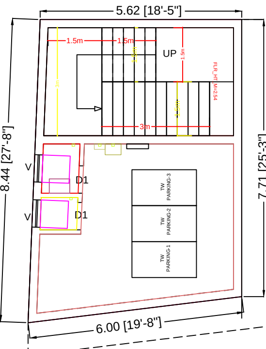
STILT FLOOR PLAN FACING SOUT
