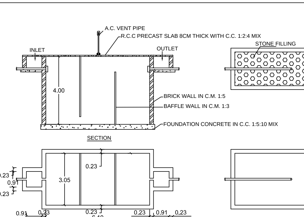
PLAN &amp; SECTION OF SEPTIC TANK &amp; DISPERSION TRENCH
