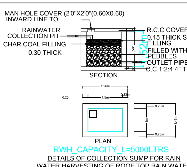
RWH_CAPACITY_L=5000LTRS
