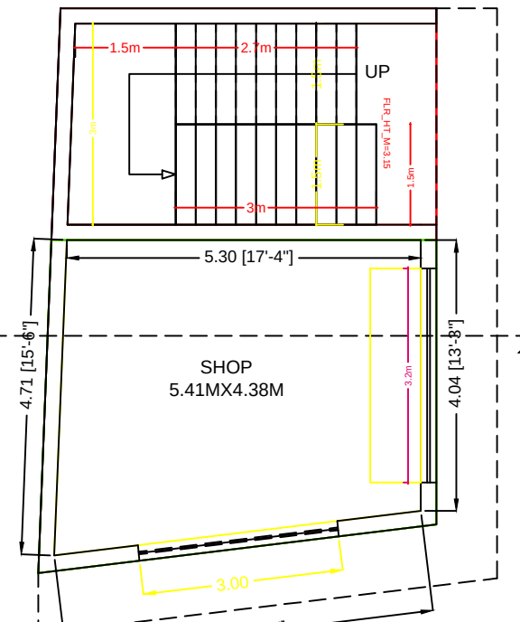
FLOOR-1 PLA
