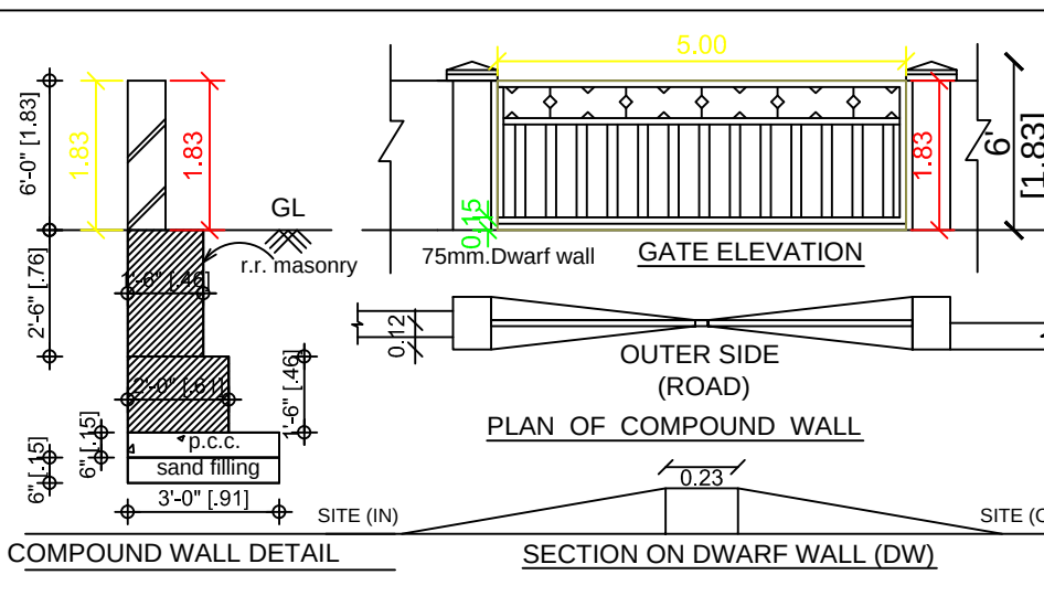
COMPOUND WALL DETAIL
