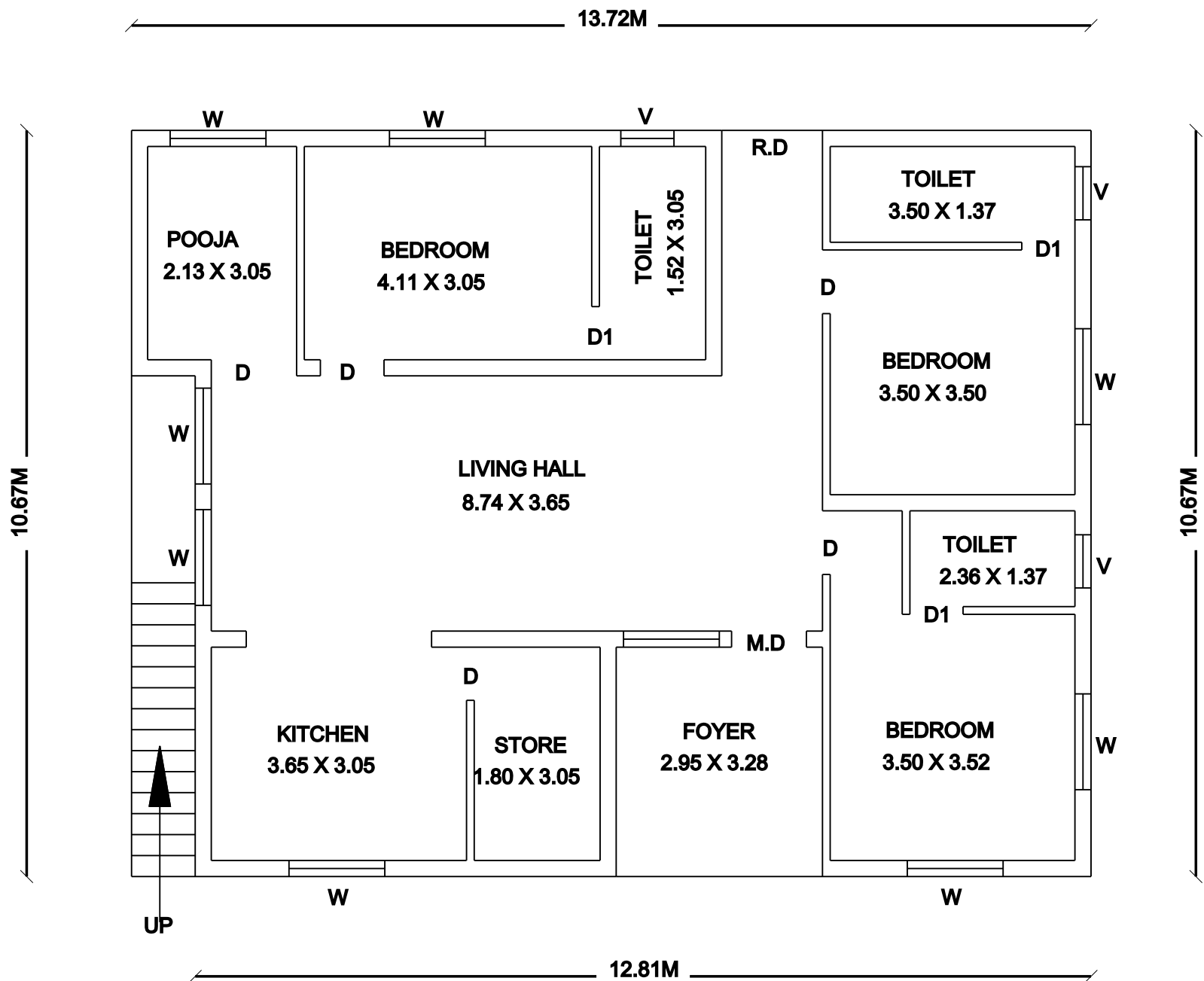
TYPICAL GROUND FLOOR PLAN
