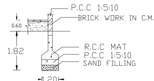
FOUNDATION DETAILS
