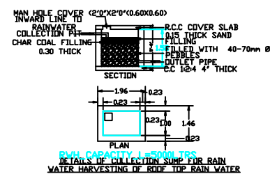
DETAILS OF COLLECTION SUMP FOR RAIN WATER HARVESTING (NTS)
