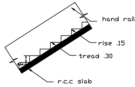
STAIR
