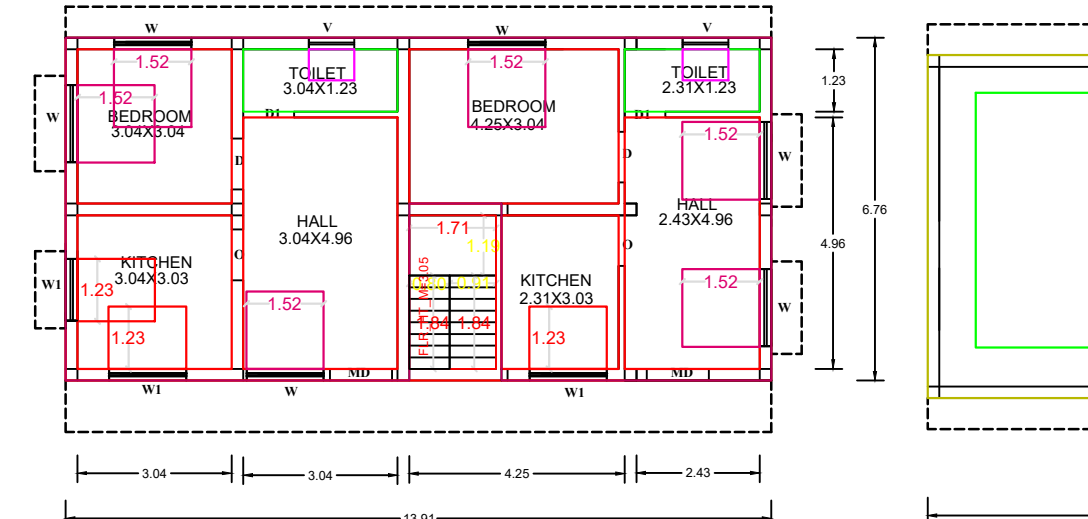
PRO.FIRST FLOOR PLAN
