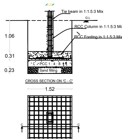
COLOUMN FOUNDATION
