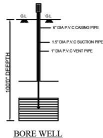
BORE WELL
