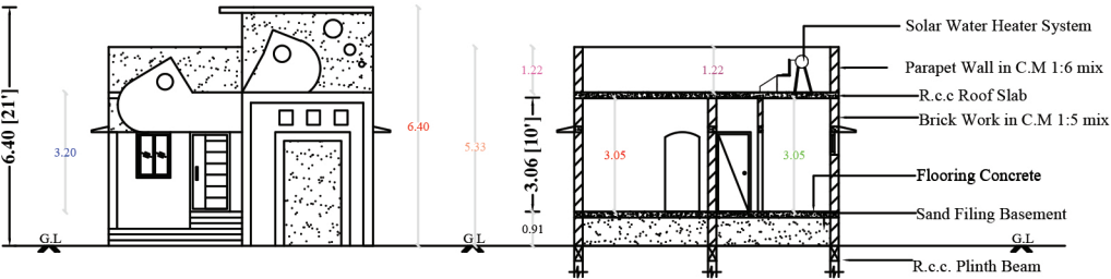
FRONT ELEVATION
