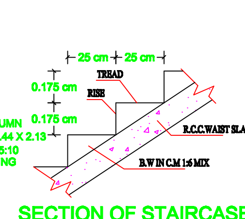
SECTION OF STAIRCASE
