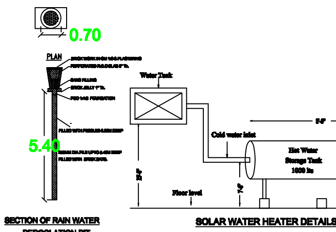
SECTION OF RAIN WATER PERCOLATION PIT
