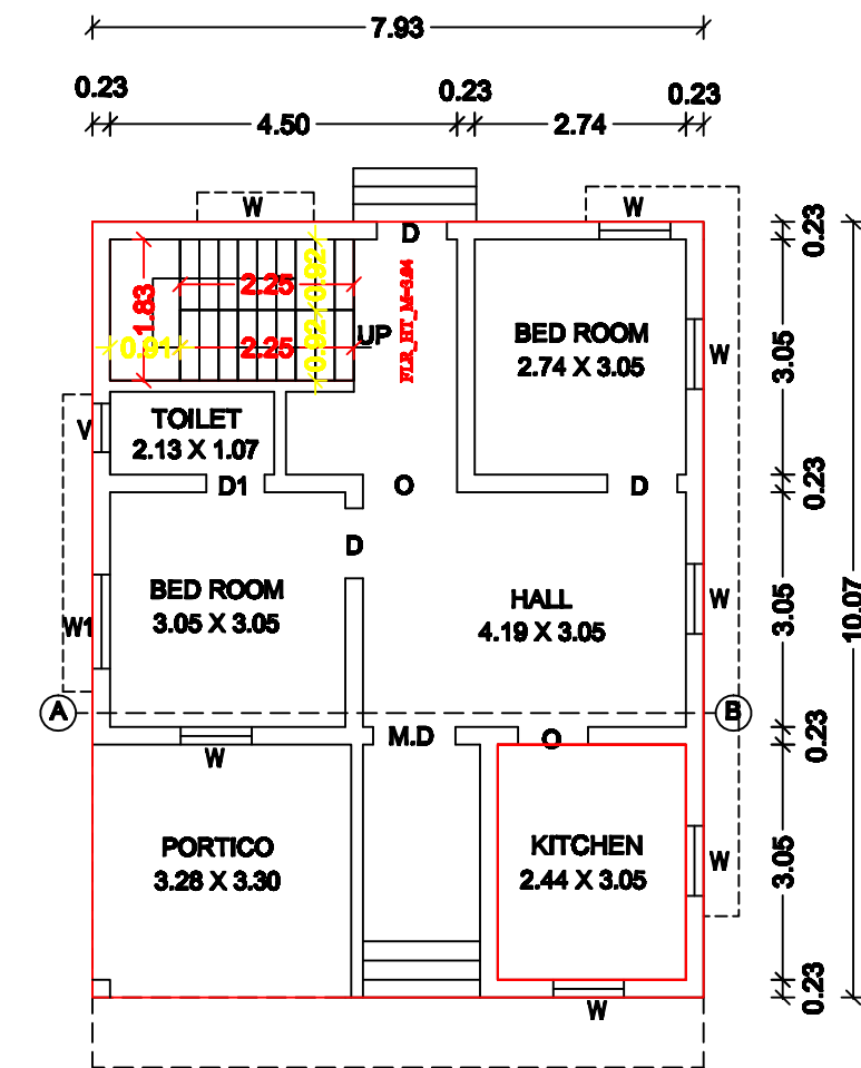
EXISTING APPROVED GROUND FLOOR PLAN
