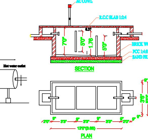
SECTION OF RAIN WATER PERCOLATION PIT
