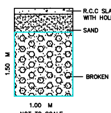
RAIN WATER HARVEST COLLECTION PIT.
