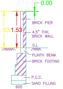
COMPOUND WALL DETAIL
