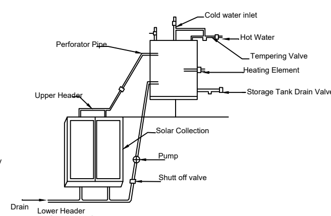
Drain Lower Header Details Of Solar Water Heater (NTS)
