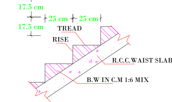
SECTION OF STAIRCASE
