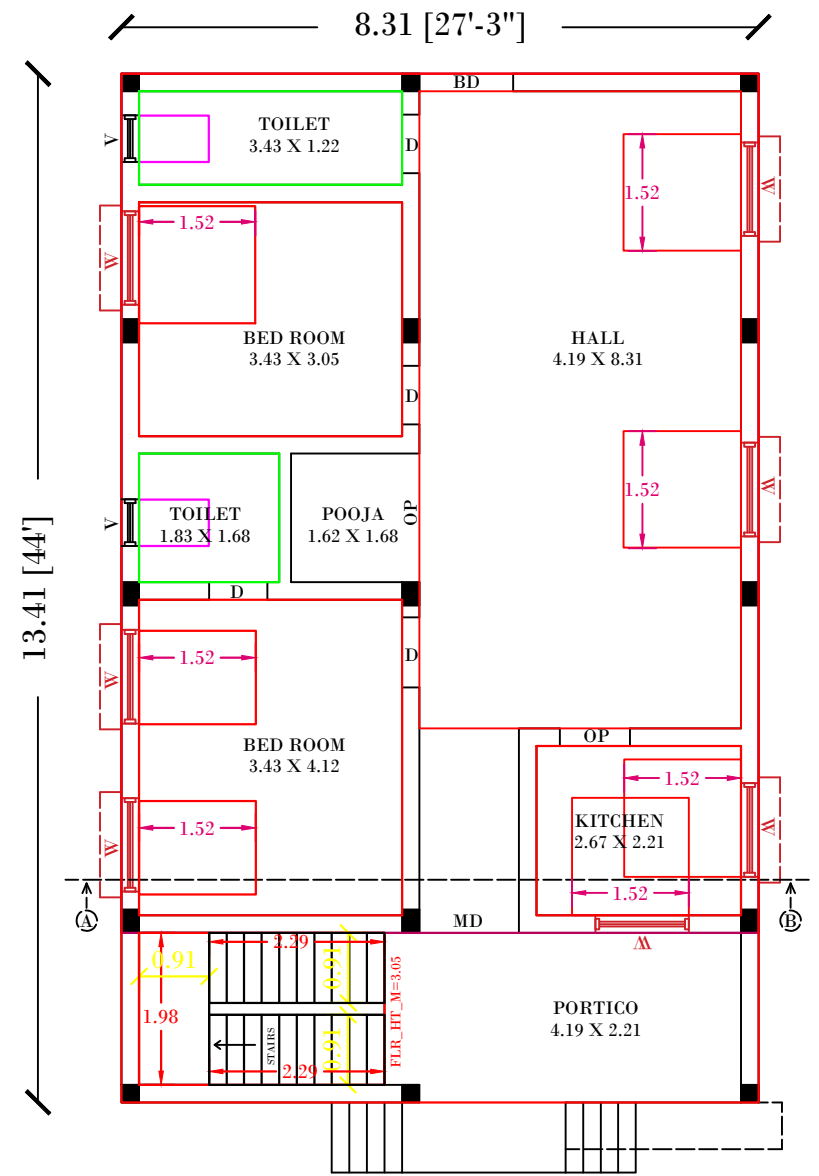
PROPOSED BUILDING GROUND FLOOR
