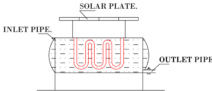
SOLAR WATER HEATER
