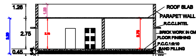
SECTION ON SS
