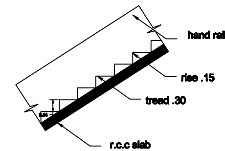
STAIR
