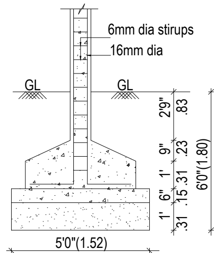
FOUNDATION DETAIL
