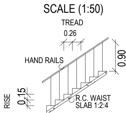
STAIRCASE DETAILS
