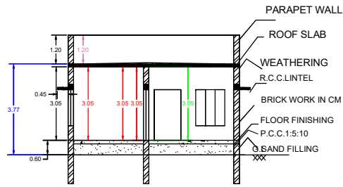
SECTION ON SS
