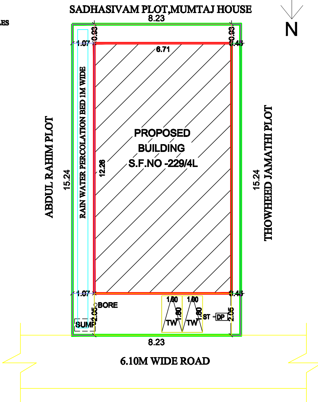
SITE PLAN
