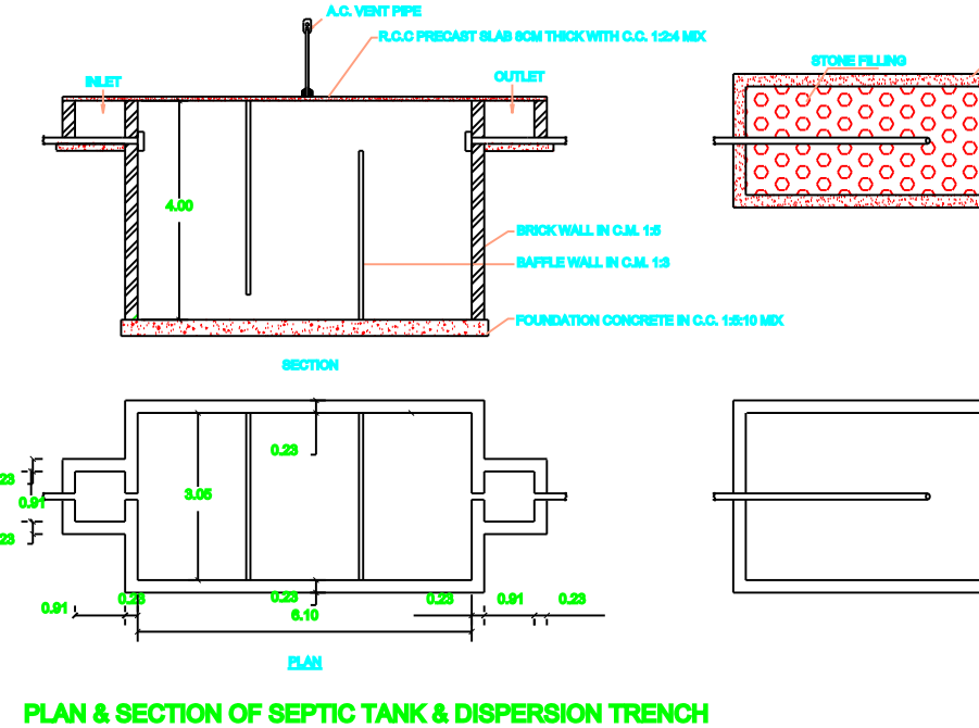
PLAN & SECTION OF SEPTIC TANK & DISPERSION TRENCH
