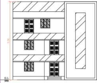
FRONT ELEVATION
