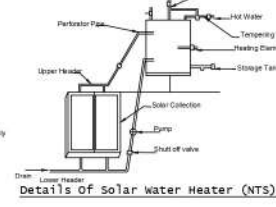
Details of Solar Water Heater (NTS)
