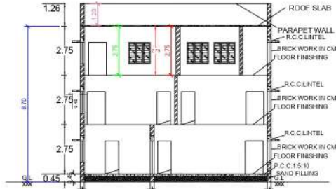
SECTION ON SS
