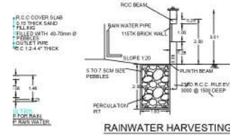
RAINWATER HARVESTING
