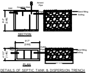
DETAILS OF SEPTIC TANK & DISPERSION TRENCH
