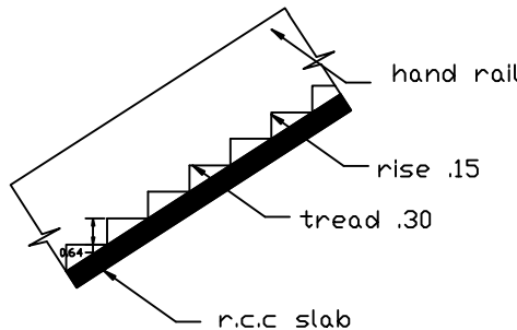
STAIR
