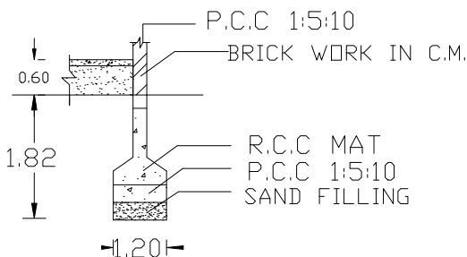
FOUNDATION DETAILS
