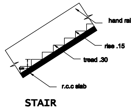
STAIR
