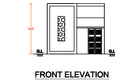
FRONT ELEVATION
