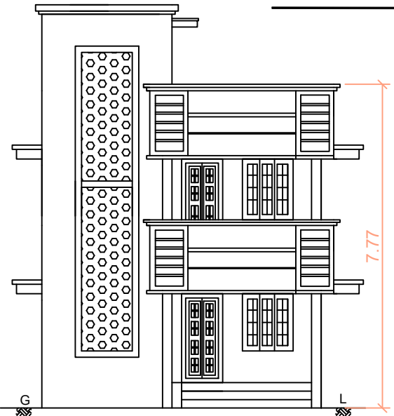
FRONT ELEVATION
