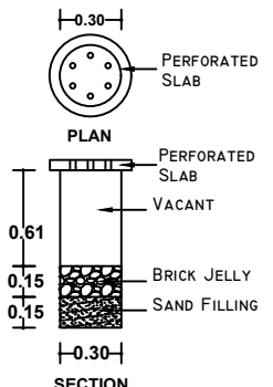
RAINWATER PERCOLATION PIT @ 3M INTERVAL
