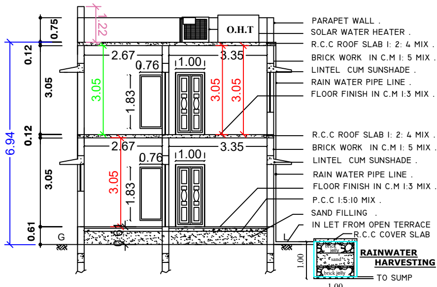
CROSS SECTION ON 'A.B'
