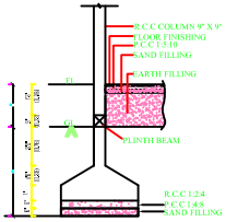
FOUNDATION DETAILS SCALE: 1"=1'-0"
