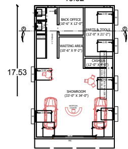
PROPOSED FLOOR PLAN
