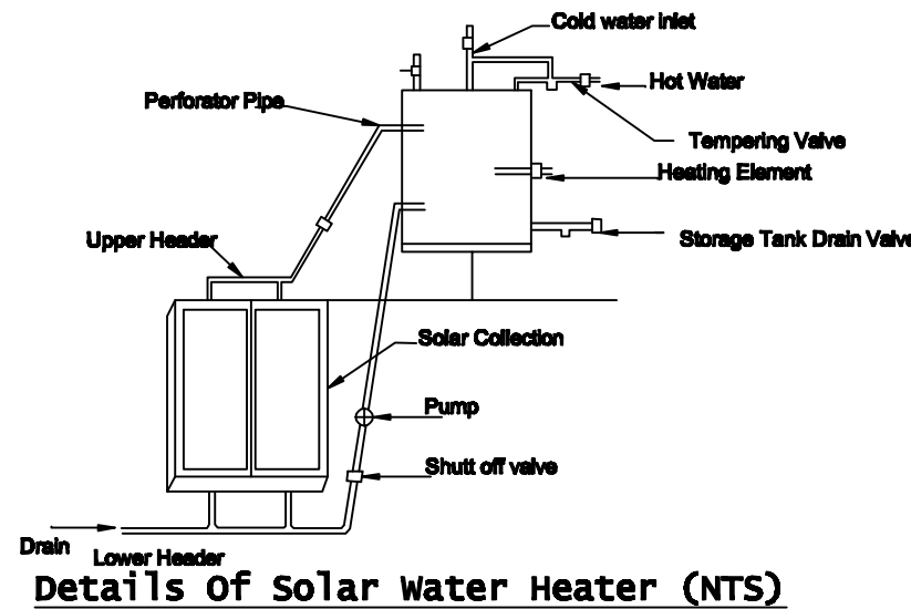
Details of Solar Water Heater (NTS)
