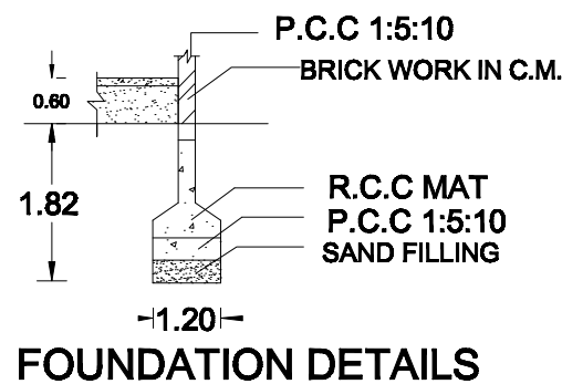
FOUNDATION DETAILS
