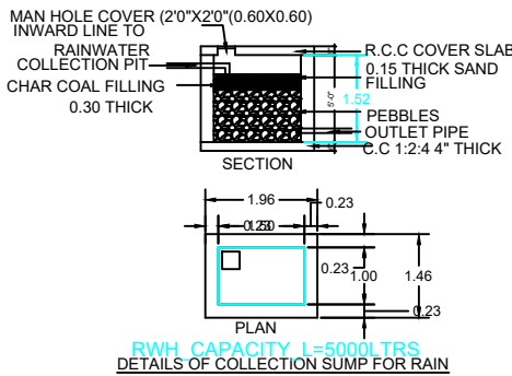
DETAILS OF COLLECTION SUMP FOR RAIN
