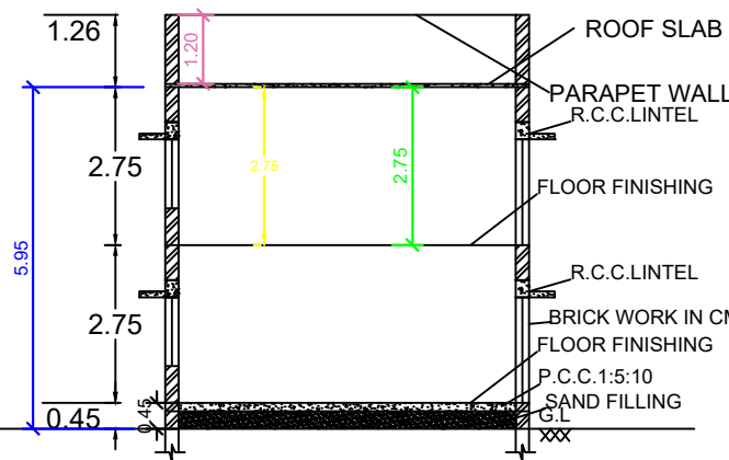
SECTION ON SS
