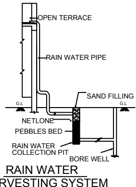
RAIN WATER HARVESTING SYSTEM
