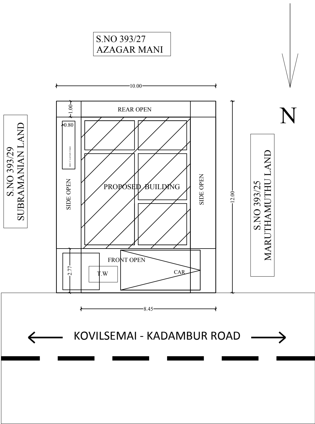
KEY PLAN
