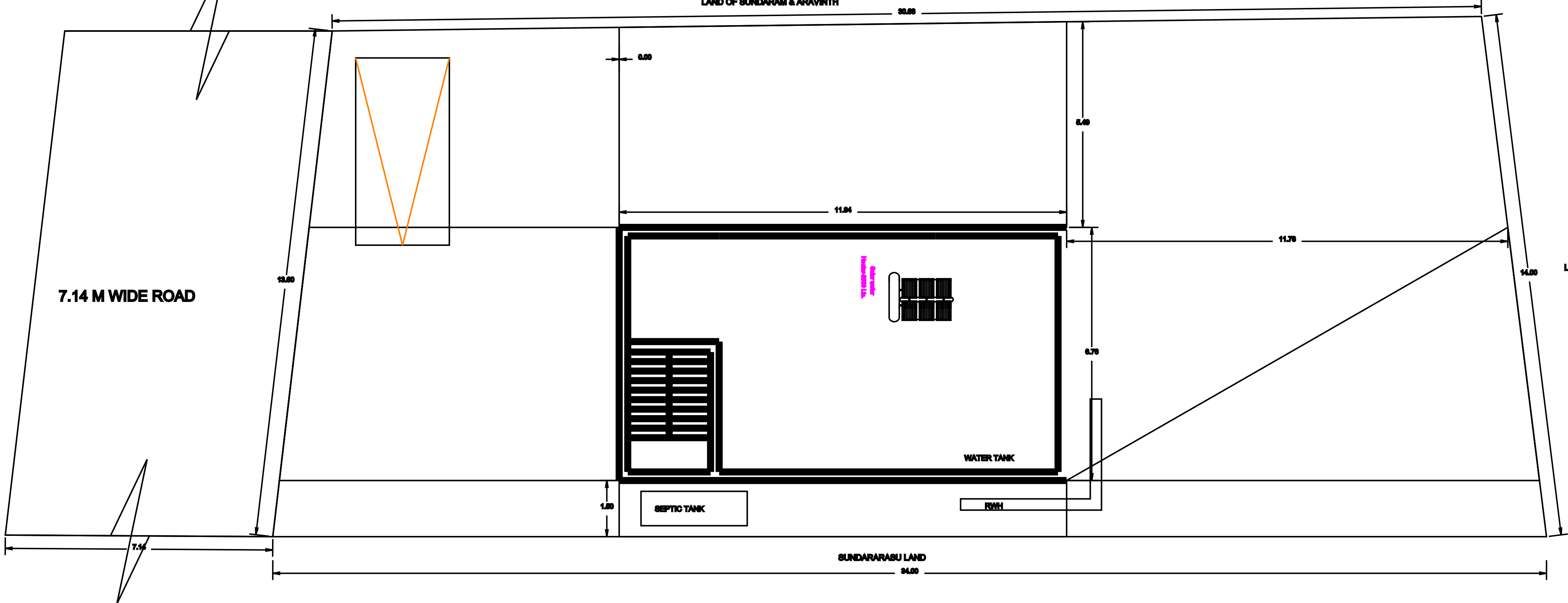
TERRACE PLAN
