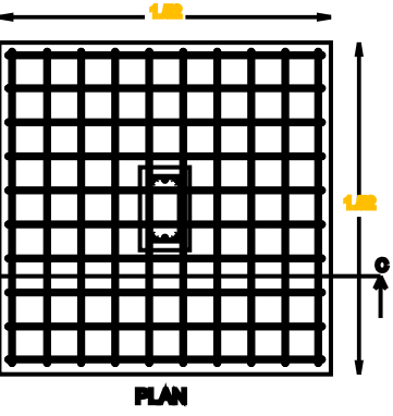
COLOUMN FOUNDATION DETAILS
