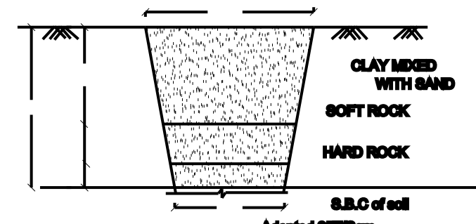
TRIAL PIT DETAILS
