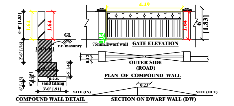
SECTION ON DWARF WALL (DW)
