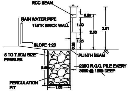
RAINWATER HARVESTING
