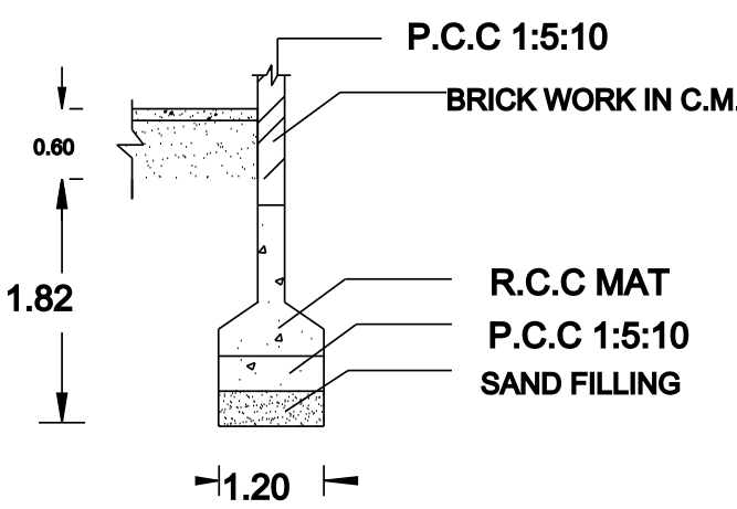
FOUNDATION DETAILS
