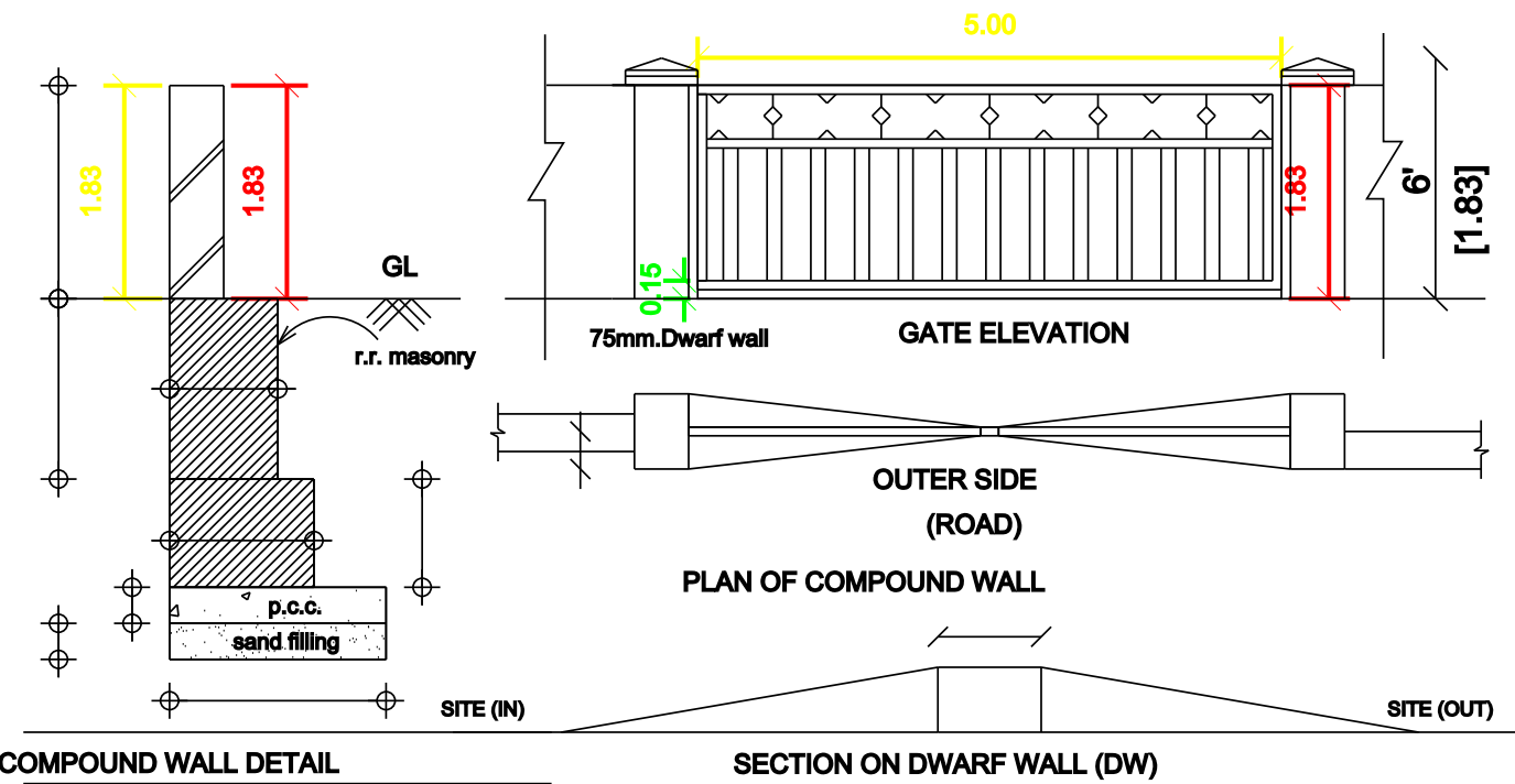
COMPOUND WALL DETAIL
