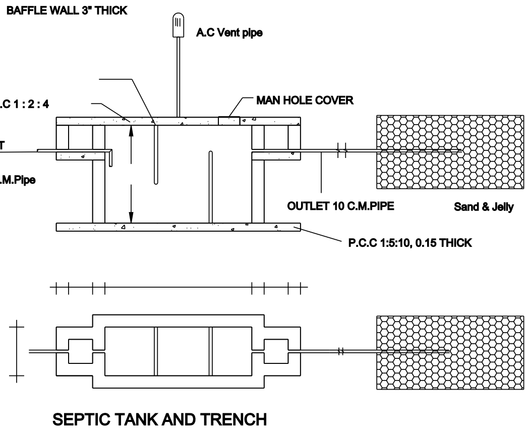
SEPTIC TANK AND TRENCH
