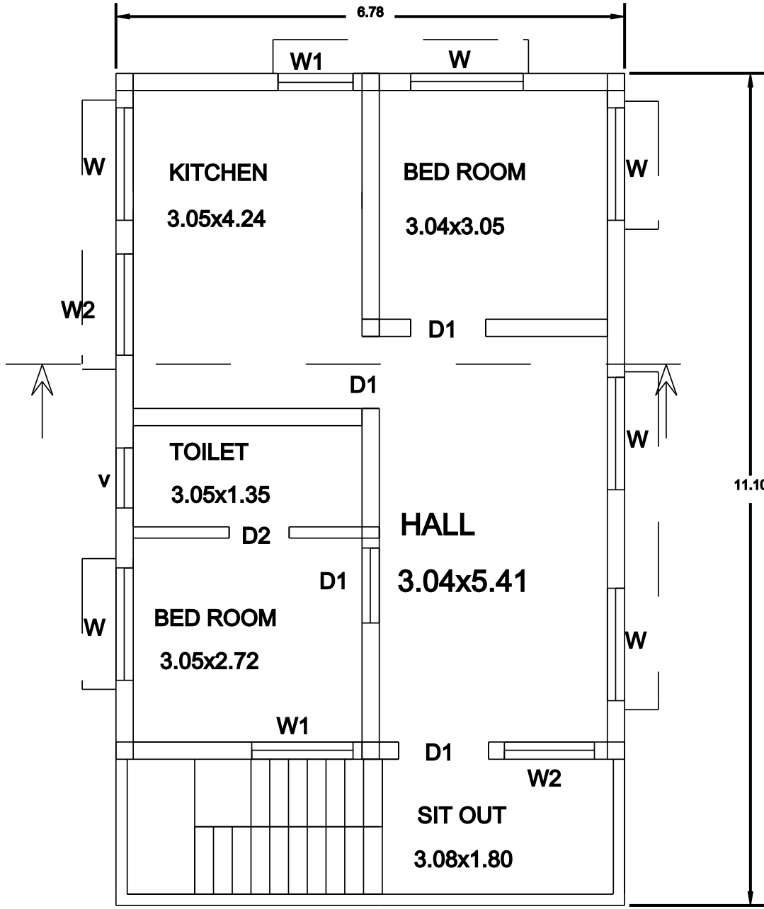
FLOOR -1
