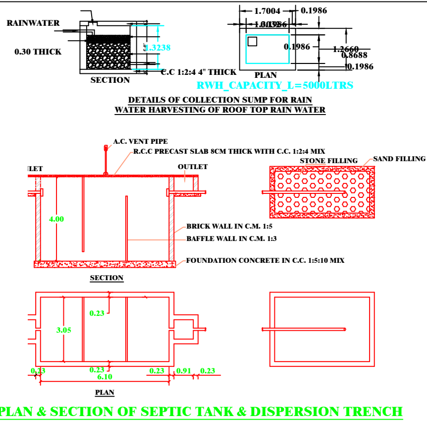
PLAN & SECTION OF SEPTIC TANK & DISPERSION TRENCH
