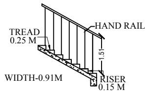
STAIRCASE DETAILS
