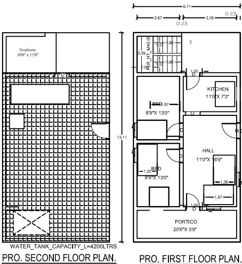
PRO. SECOND FLOOR PLAN.
