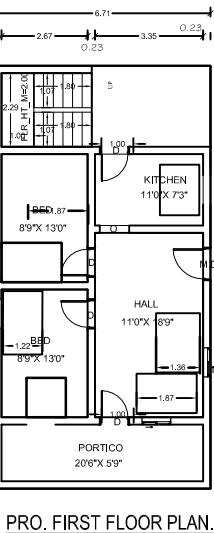
PRO. FIRST FLOOR PLAN.
