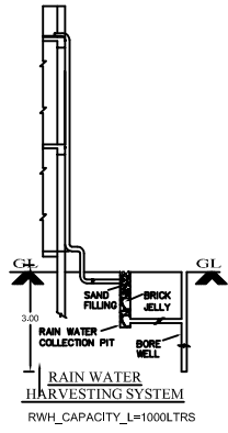
PERCOLATION PIT
