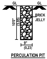
PERCOLATION PIT
