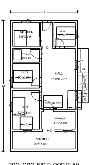
PRO. GROUND FLOOR PLAN.
