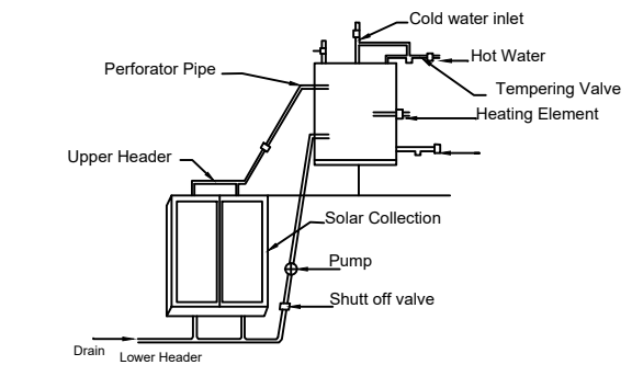
Details of solar water Heater (NTS)
