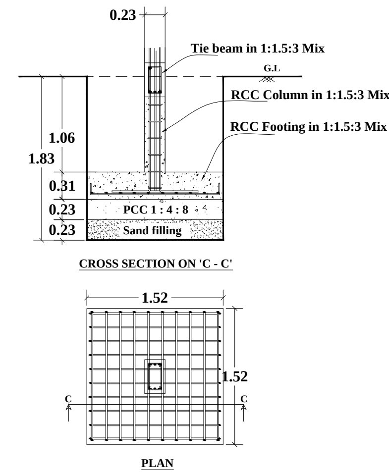
COLOUMN FOUNDATION DETAILS-"AB"
