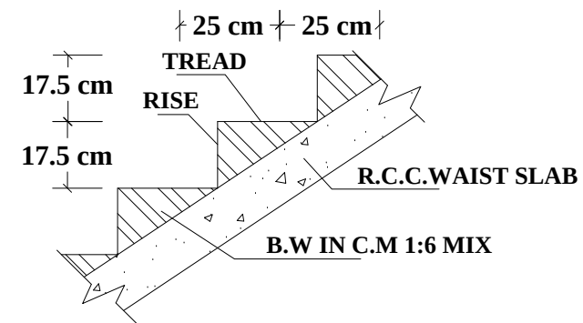
SECTION OF STAIRCASE
